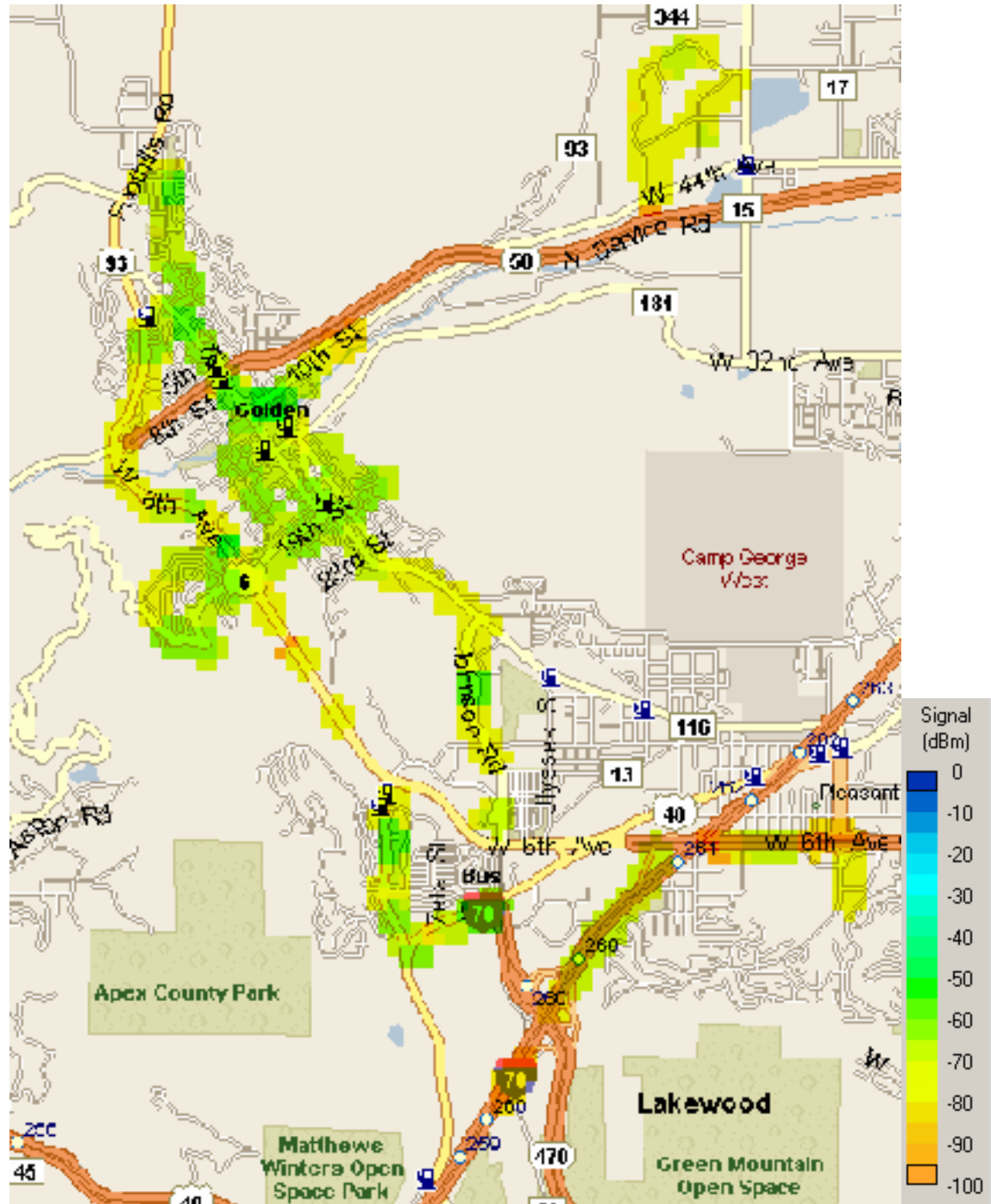
Figure C-2. Signal Strengths of Existing Access Points along the Test Route.
