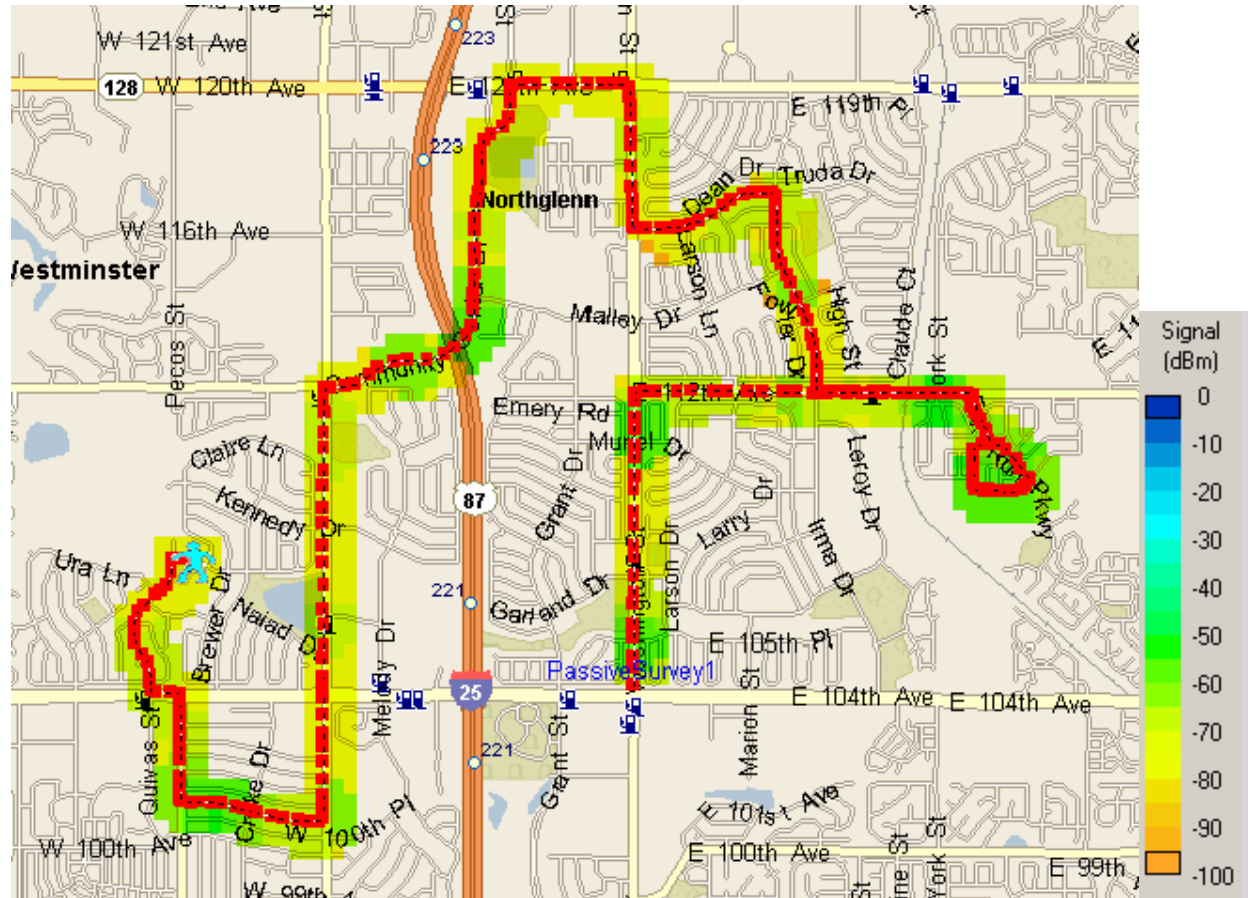
Figure C-2. Signal Strengths of Existing Access Points along the Test Route.
